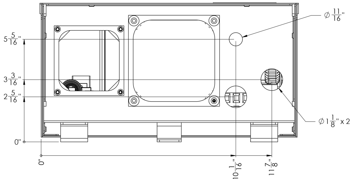
FRONT TYPE 1 NEMA 3R
