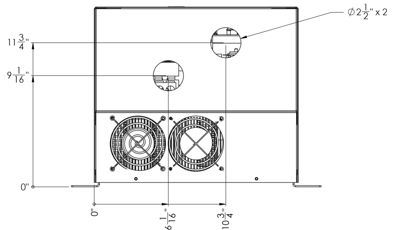
FRONT NEMA 1
