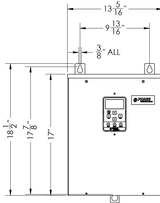
FRONT TYPE 1 NEMA 3R
