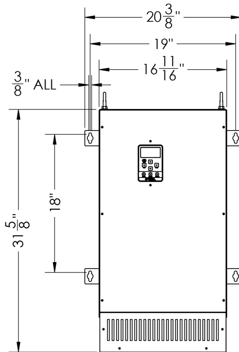
FRONT NEMA 1
