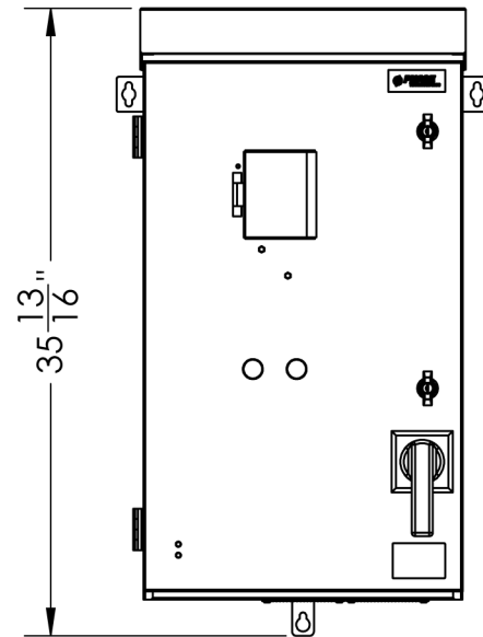
FRONT - 3R AND BREAKER
