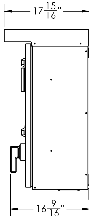
SIDE - 3R AND BREAKER
