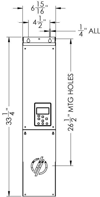
FRONT NEMA 1
